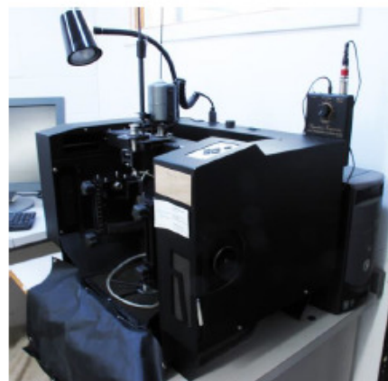
Actual photo of the machine in my shop with DELL CPU tower behind the machine and gold foil stylus attached to top of machine
